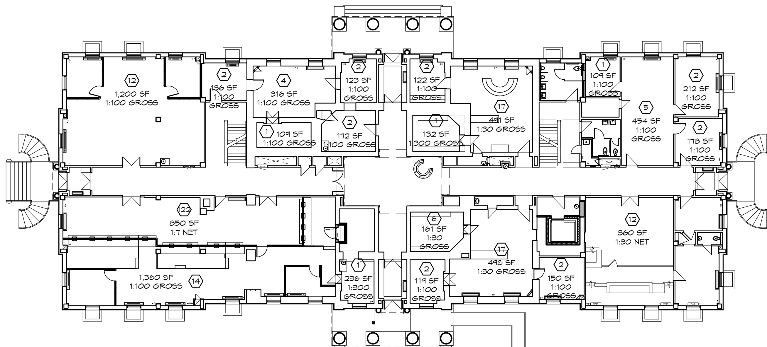
FIRST FLOOR
